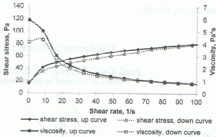
Figure 4. Rheological behaviour of the olive - palm oil pre-emulsion under frequency sweep and flow test
