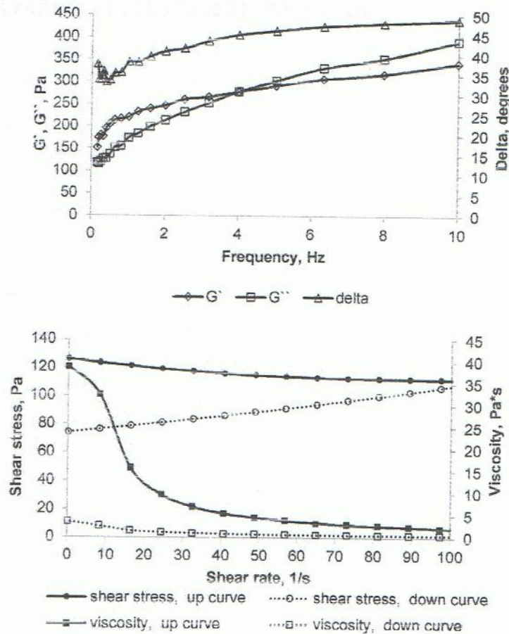
Figure 2. Rheological behaviour of palm oil under frequency sweep and flow tests
