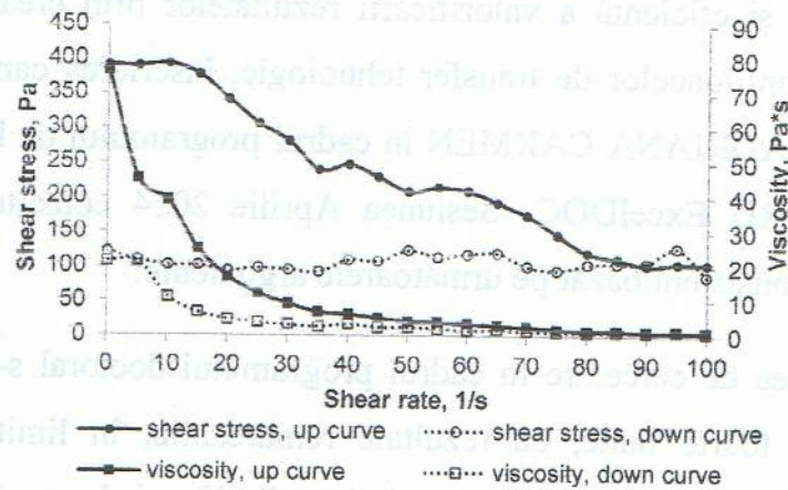
Figure 3. Rheological behaviour of pork backfat under frequency sweep and flow tests
